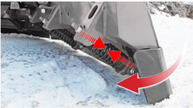
Cutting edge with trip springs
