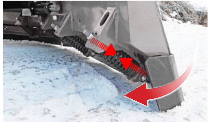
Cutting edge with trip springs
